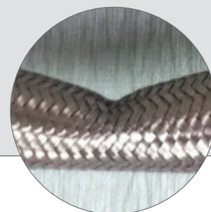
Kinking Damage
